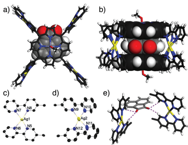
Figure 2. The X-ray crystal structure of [3C(2)(CH_3OH)_2] \cdot (CF_3CO_2)_4 . CF_3CO_2^- anions and hydrogen atoms of CH_3OH coordinating to Zn^{II} are omitted for clarity. Ag yellow, Zn light purple, C black (for 2^{4+} and CH_3OH ), C gray (for 3 ), N blue, O red, H white. 3 (a) as well as 3 and the porphyrin rings (b) are shown as a space-filling model. The structures in c) and d) are shown in an ellipsoidal model. The others are shown as a stick model. Top view (a) and side view (b) of [3C(2)(CH_3OH)_2]^{4+} . c,d) Bis(bpy) Ag^I units, in which Ag^I centers adopted a four-coordinate distorted square-planar geometry. Thermal ellipsoids are set at 50% probability. Hydrogen atoms are omitted for clarity. See the Experimental Section for selected bond lengths and angles. e) Hydrogen bonds (purple dashed line) between C–H bonds of pyridyl groups in 2^{4+} and carbonyl oxygen atoms of 3 .
